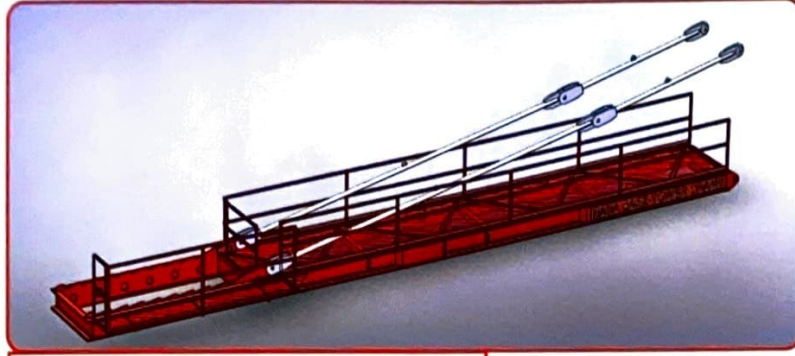
Kuyruk / Counter Jib
