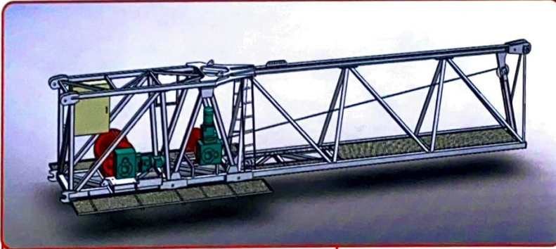
Ana Bom / Main Jib
