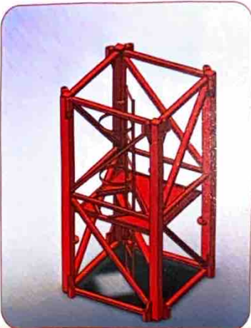
2,95 m Boyunda MAST MAST With 2.95 m Height
